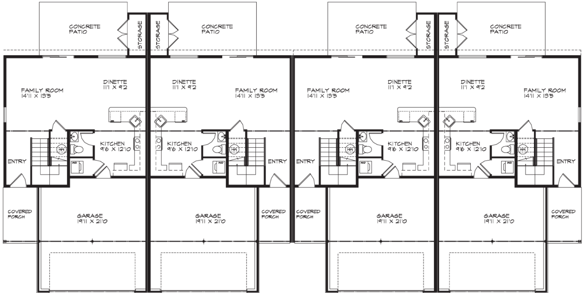
FIRST FLOOR
